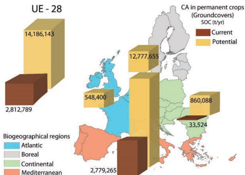
Fig. 9. Current and potential SOC fixed by groundcovers compared to systems based on soil tillage in France, Germany, Italy, Netherlands, Poland, Spain and the United Kingdom.
