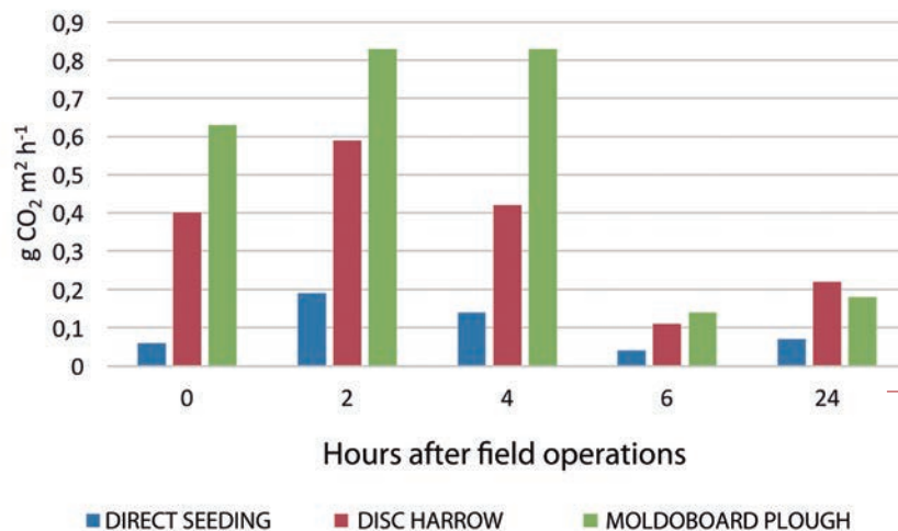
Fig. 4.3. Increase of CO 2 emissions per hour during the tillage operations on the soil in the different cropping systems. (Each value represents the average of 14 readings). Source: Carbonell-Bojollo et al., (2011).
