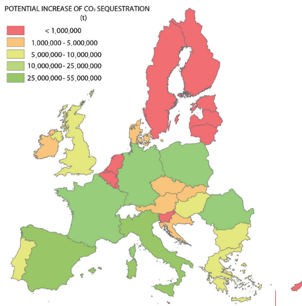
Fig. 4.10. Potential increase (potential – current) of CO 2 sequestration in Europe through CA.
